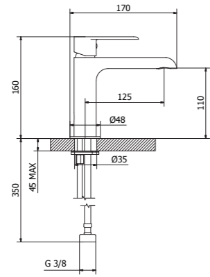
8X301 Wash basin mixer
