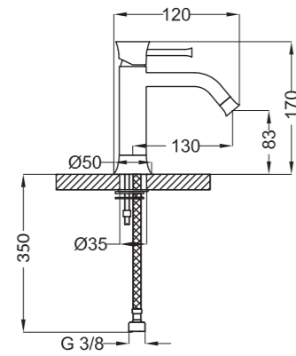
8Y301 Wash basin mixer
