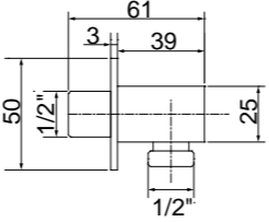
QUADRA Prese acqua Wall connection for shower Штуцер 1/2"
